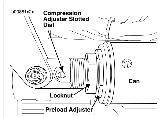
Figure 5. Preload and Compression Damping Adjustment
